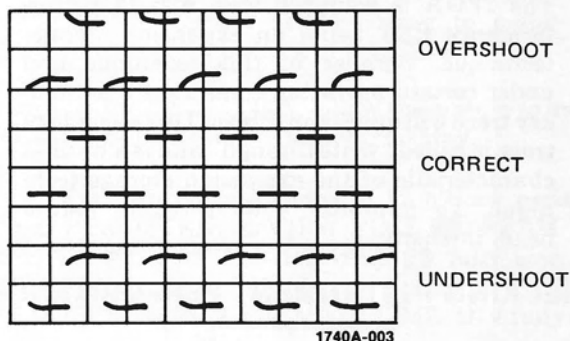
Figure 3. Probe Compensation
