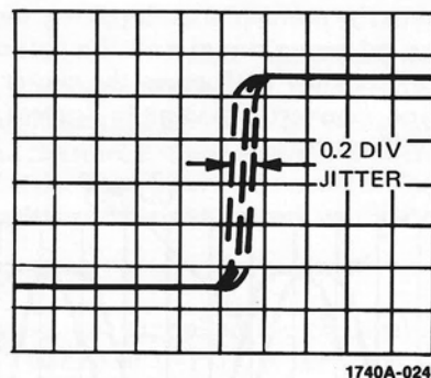
Figure 22. Pulse Jitter Measurement
