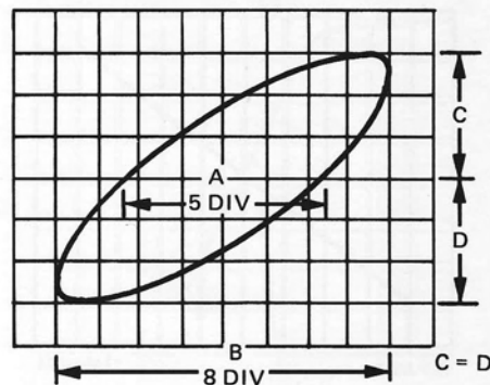
Figure 25. A VS B Phase Measurement
