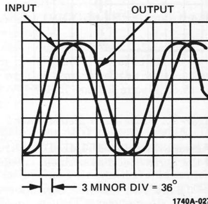
Figure 24. Phase Difference Measurement
