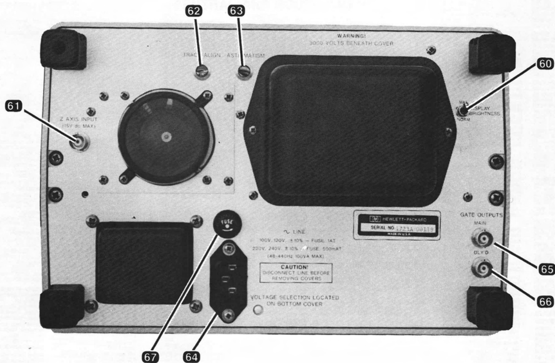
Figure 32. Front and Rear-panel Controls and Connectors 49
