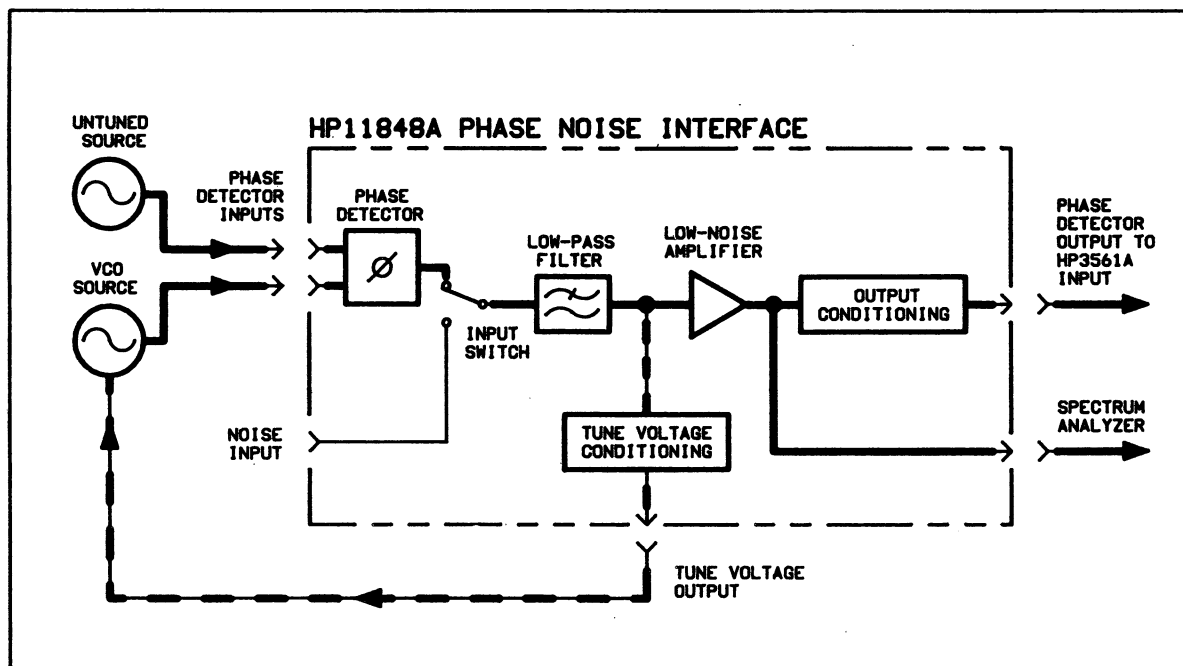
Figure 5. Noise Measurement with the Internal Phase Demodulator
