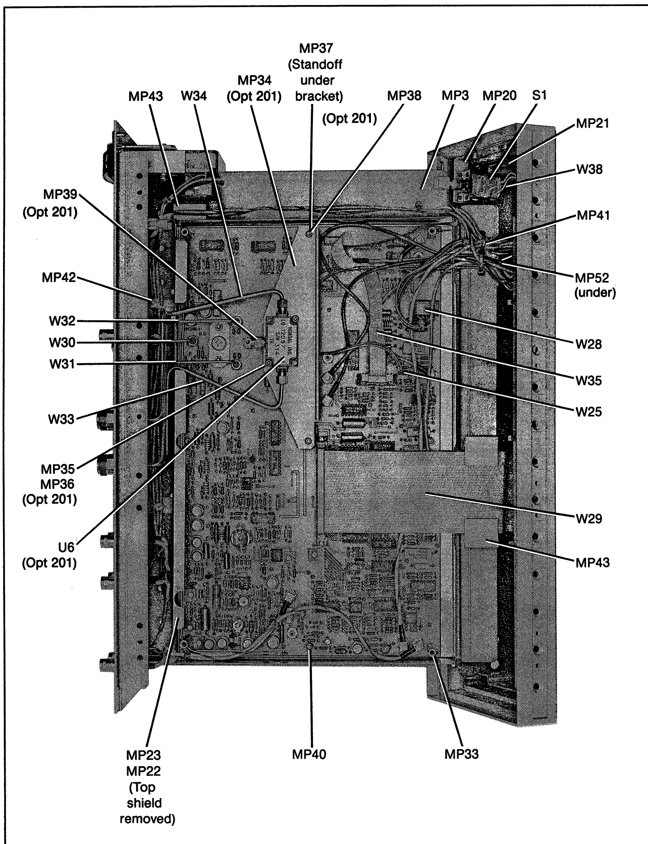
Figure 9. Parts and Cable Identification (Top View)
