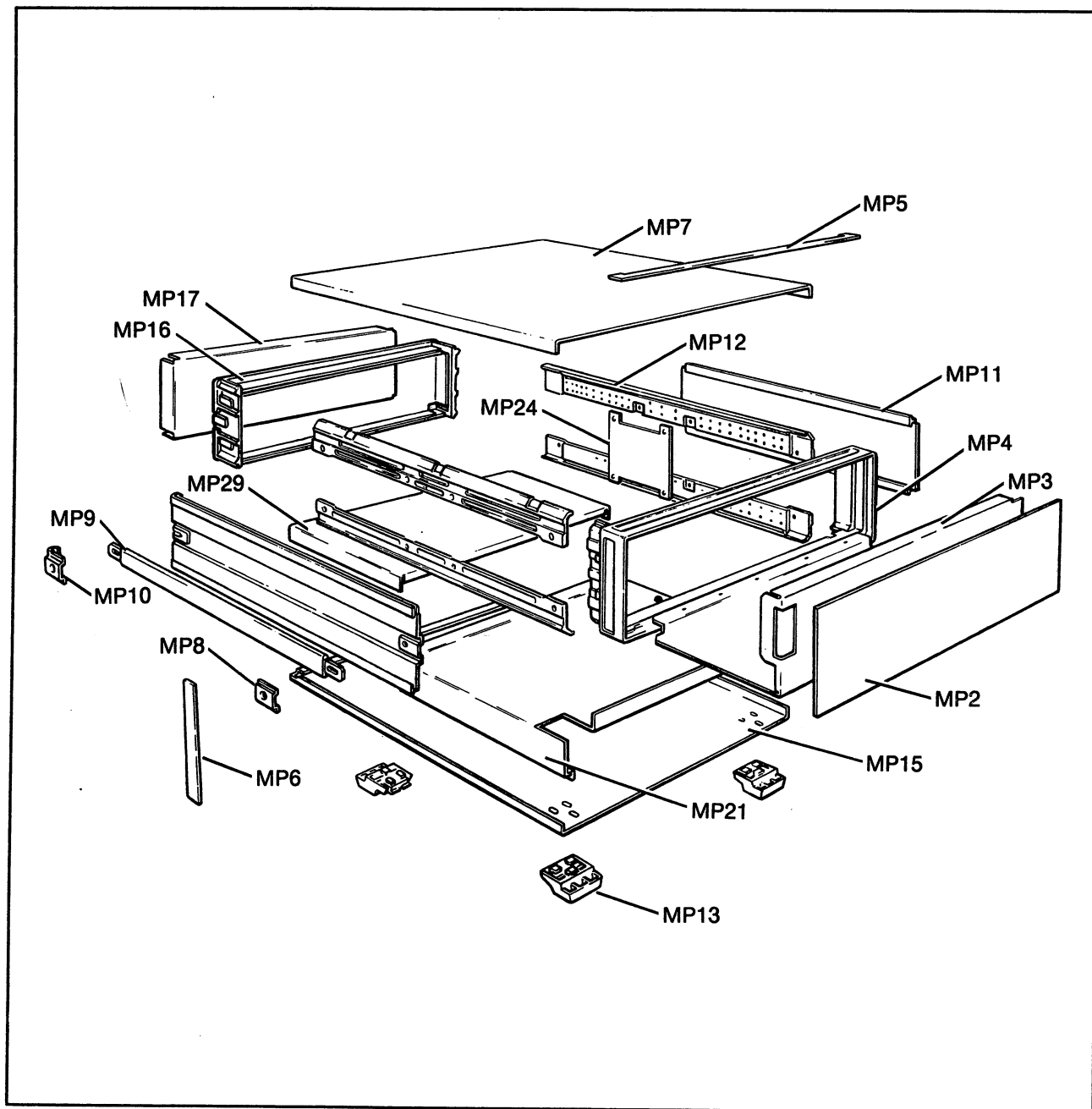
Figure 6. Cabinet Parts
