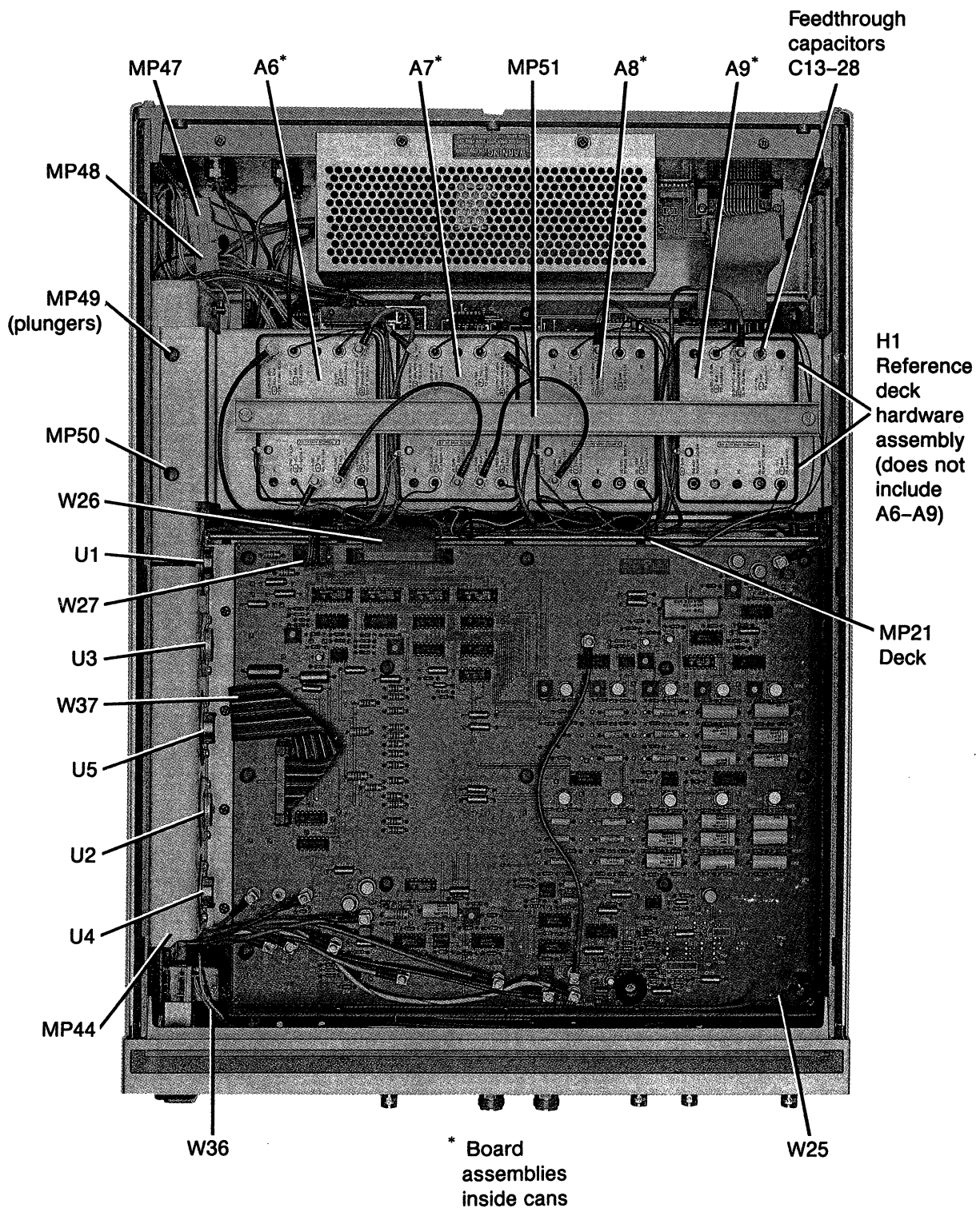
Figure 8. Parts and Cable Identification (Top View)
