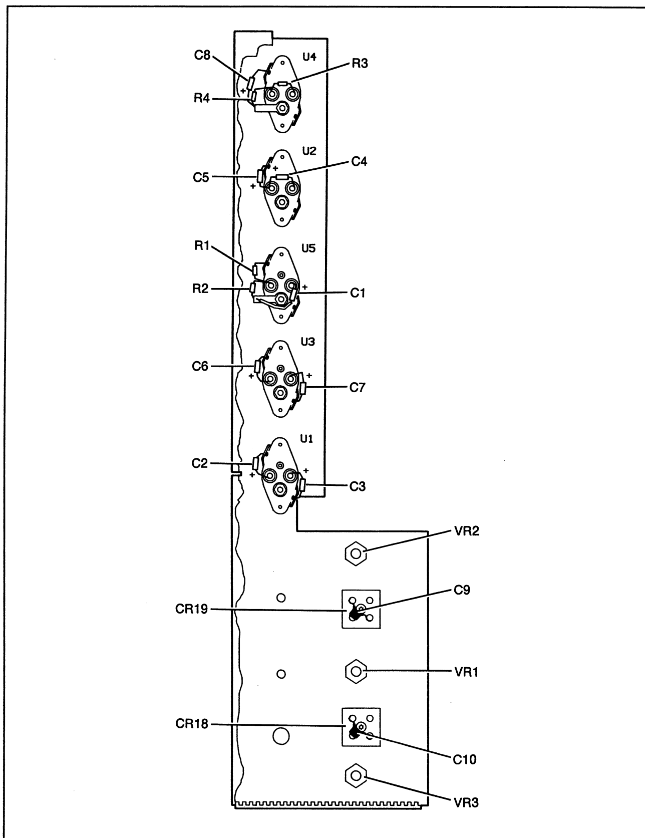
Figure 11. Parts Identification (Regulator Assembly)
