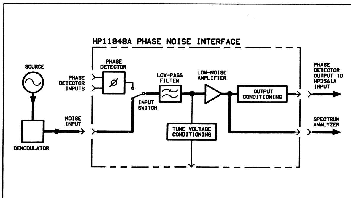
Figure 4. Noise Measurement with an External Demodulator
