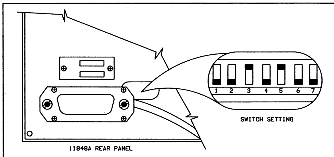
Figure 3. HP-IB Address Switch
