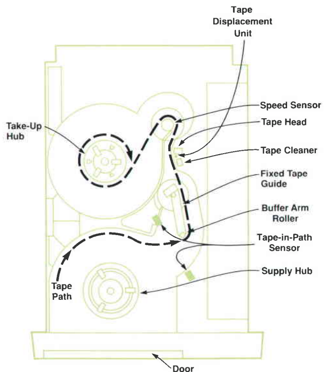
Fig. 2. HP 7980A tape path components.
