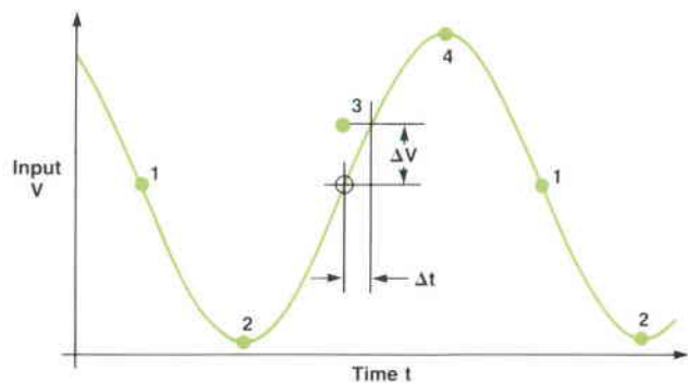
Fig. 4. Effect of uneven sample timing in an interleaved system.
