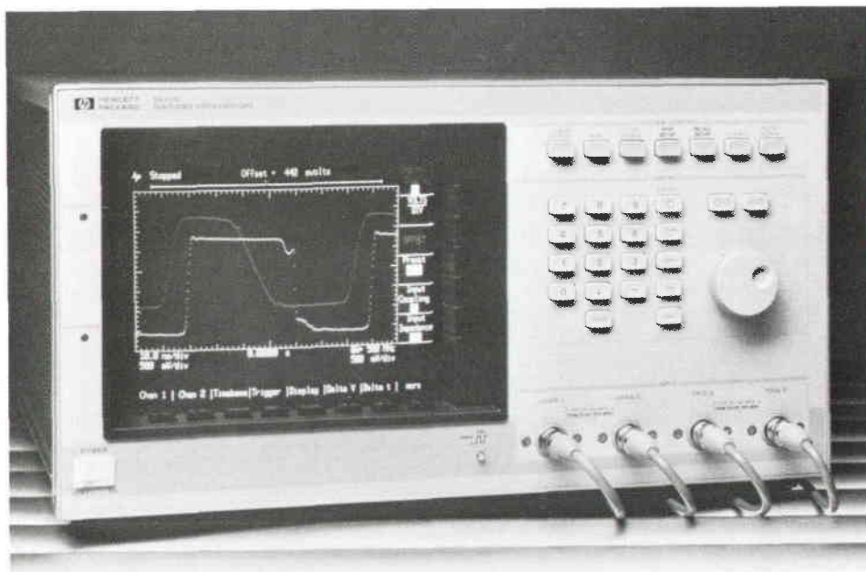
Fig. 1. The HP 54111D Digitizing Oscilloscope can sample high-speed transient signals at 1 gigasample/s. It features a 250-MHz single-shot bandwidth and a 500-MHz repetitive bandwidth with up to 8 bits of vertical resolution.
