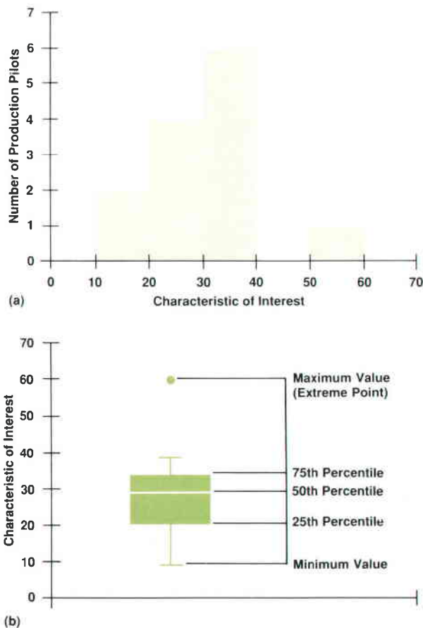
Fig. 1. (a) Histogram and (b) boxplot for the same data.
