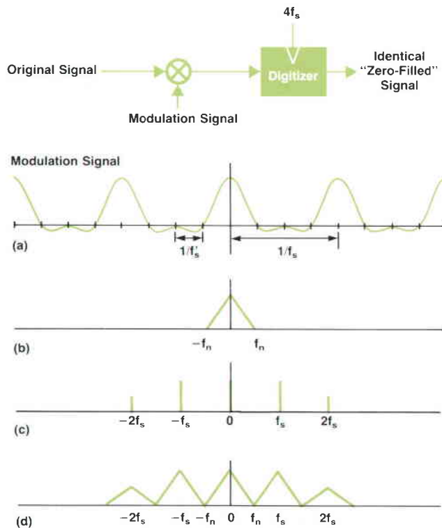
Fig. 5. (a) Multiplying input signal by modulation signal. Original spectrum (b) convolved with modulation signal spectrum (c) gives a "zero-filled" spectrum (d). The result after sampling at f'_s is identical to Fig. 4e.
