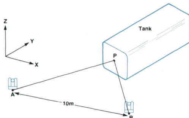
Fig. 1. A small change in large object dimensions such as the bulge in a tank wall before and after being filled can be easily measured with the 3820A Coordinate Determination System.
