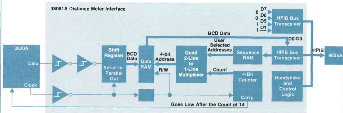
Fig. 2. Block diagram of the electronics of the 38001A Distance Meter Interface.
