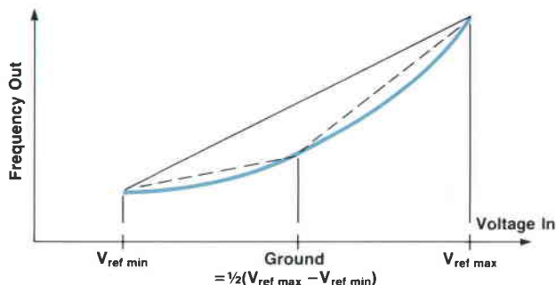
Fig. 2. Typical voltage-to-frequency converter transfer functions are nonlinear. In the 5335A counter, the ends and mid-point of the transfer function are measured in a microprocessor calibration routine performed on each measurement. Then a two-segment linear approximation of the curve is used to reduce the conversion error.
