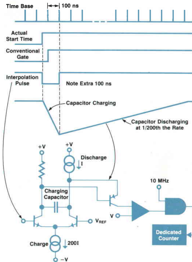
Fig. 3. The 5335A achieves high resolution (near 1 ns) through interpolation. The time between the true opening of the gate and the conventional opening of the gate—plus 100 ns—is used to charge C_i . The capacitor is then discharged at about 1/200th of the charge rate to stretch the time interval so that it can be measured to high resolution by a conventional dedicated counter.
