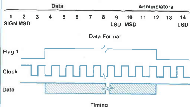
Fig. 1. Data format and timing for the output of the 38001A. The annunciators indicate to the controller what type of data is being sent.
