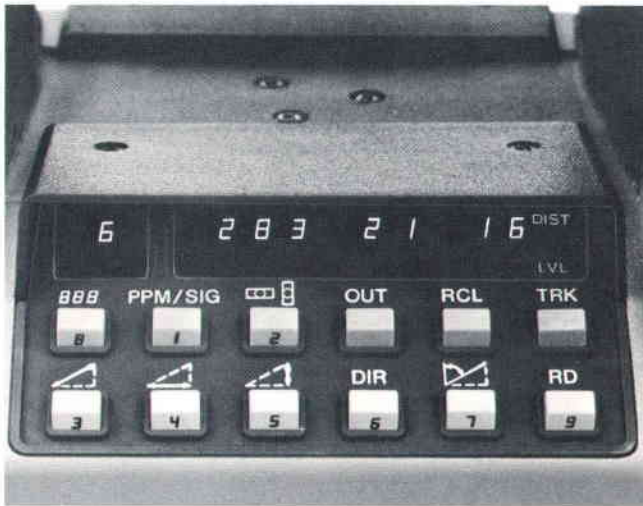
Fig. 4. Close-up view of 3820A keyboard and display. There are two of these units, one on each side of the instrument, for user convenience.
