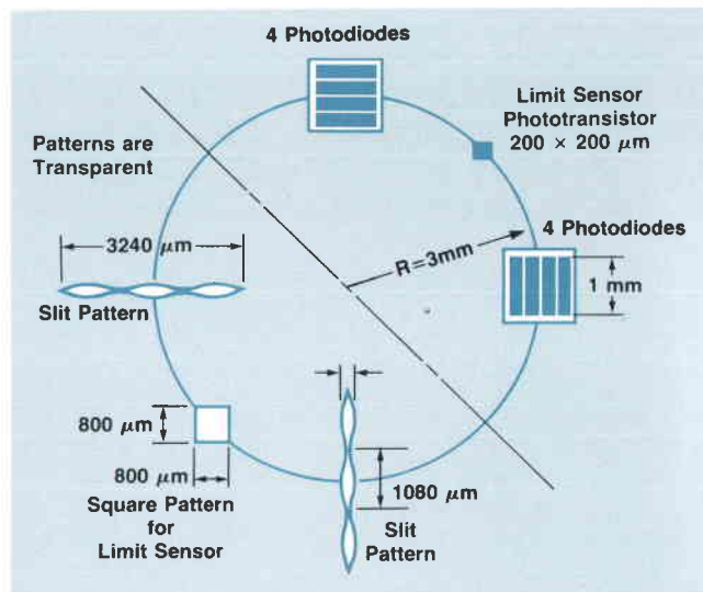
Fig. 10. Arrangement of slit patterns and optical sensors for tilt meter. The tilt position measurement technique is the same as that used for angle measurement.
