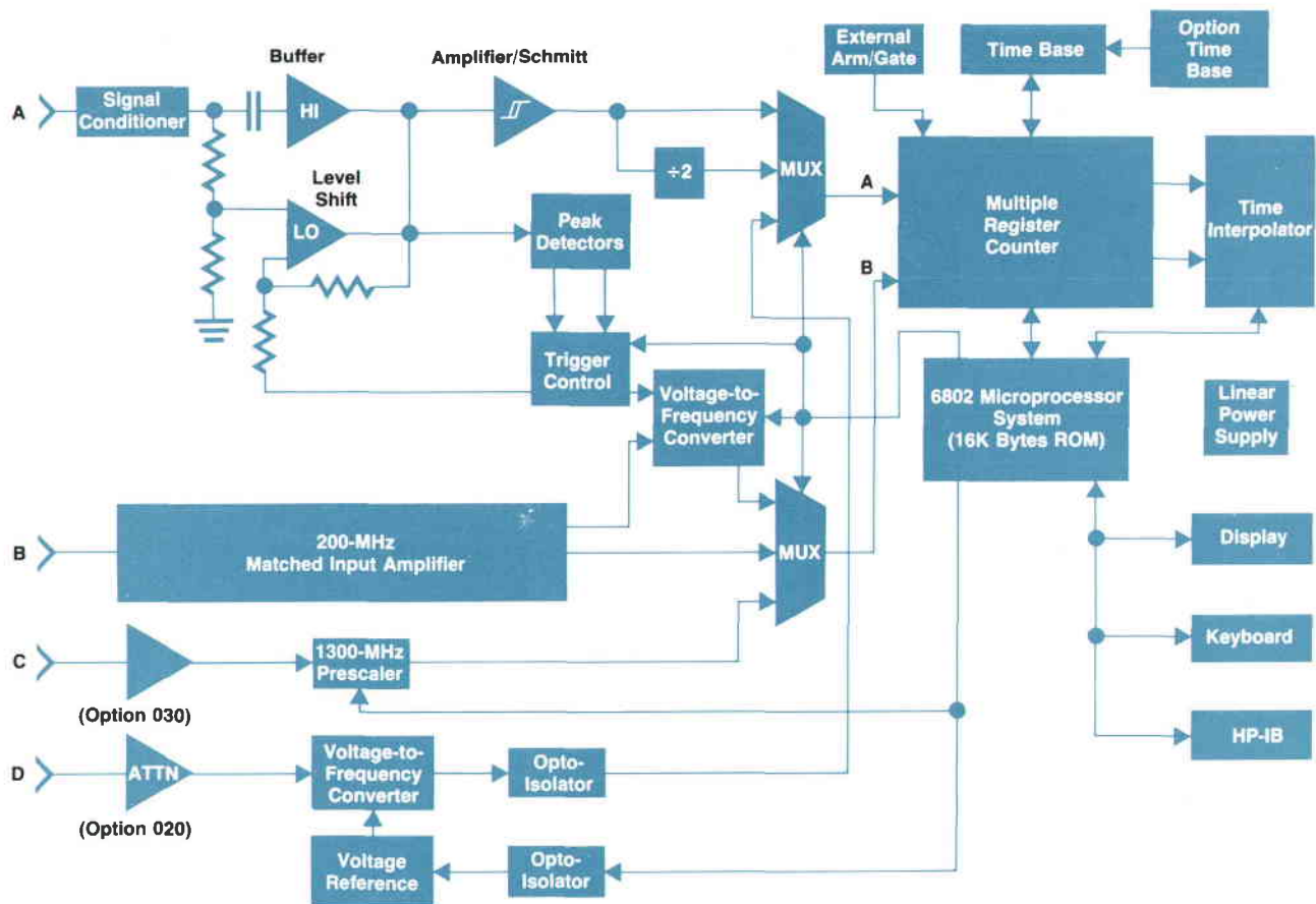
Fig. 2. Advanced architecture of Model 5335A Universal Counter is based on two main integrated circuits—the multiple register counter and the microprocessor. All other blocks support these two.
