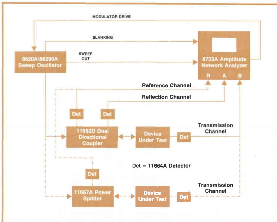
Fig. 3. System for simultaneously measuring transmission and reflection parameters.
