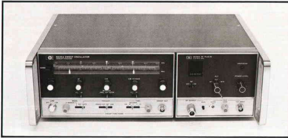
Fig. 1. Model 86290A is a new RF plug-in for Model 8620A Sweep Oscillator. Four frequency bands are selectable by front-panel controls: 2-6.2, 6-12.4, 12-18, and 2-18 GHz. The combination is the most compact broadband sweeper currently available.
