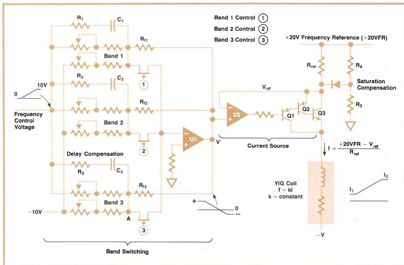
Fig. 4. YIG driver circuits provide the linear current ramps that tune the YIG resonators. The drivers also compensate for magnetic saturation and delay in the YIG magnets.
