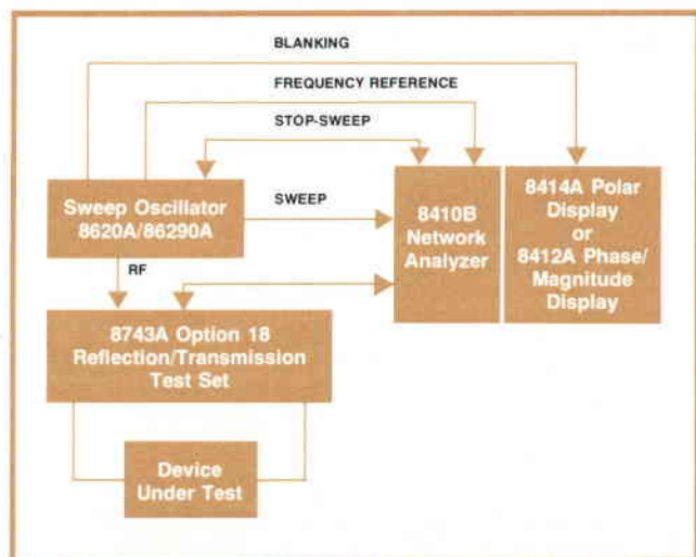
Fig. 1. A 2-to-18-GHz scattering parameter measurement system.
