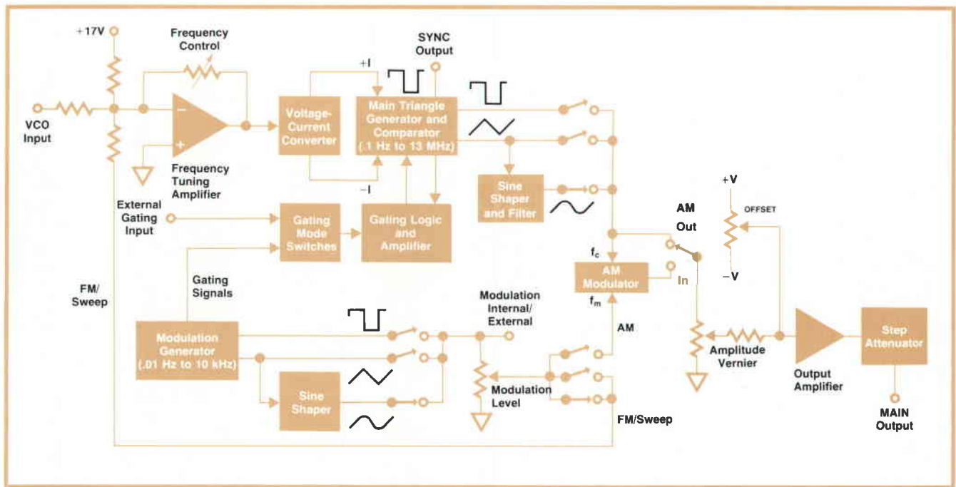
Fig. 5. Simplified diagram of the Model 3312A Function Generator. The frequency of the main generator is controlled by a front-panel knob, by the modulation generator, by an external voltage, or by any combination of the three.
