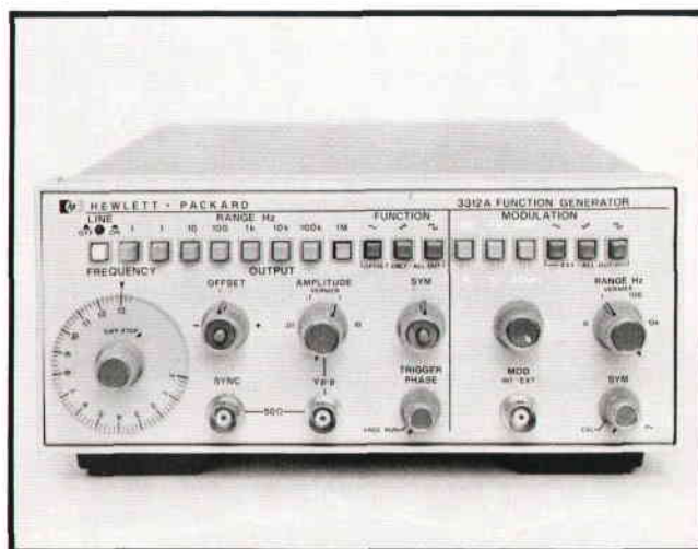
Fig. 1. Model 3312A Function Generator combines two signal sources to produce a wide variety of test signals. Total frequency coverage is from 0.01 Hz to 13 MHz.
