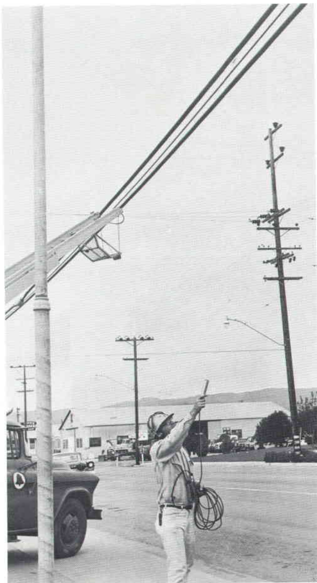
Ultrasonic detection of leaks in pressurized telephone cables has eliminated old-fashioned soap-bubble method. Leaks can usually be heard from the ground, often from a truck driving along the cable path. Translator responds only to sounds between 36 kHz and 44 kHz and is not affected by audible traffic noises.
