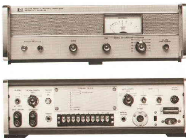
Logic and automatic alarm circuits are built into new ac-powered Model 4950A Ultrasonic Translator for automated ultrasonic production testing. Instrument responds either to ultrasonic signal or to its integral, and closes a relay whenever signal or integral exceeds level set with input attenuator.
