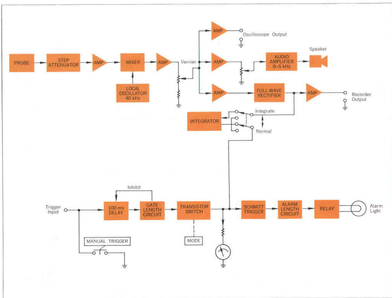
Block diagram of Model 4950A Ultrasonic Translator, showing logic and alarm circuits for production testing.
