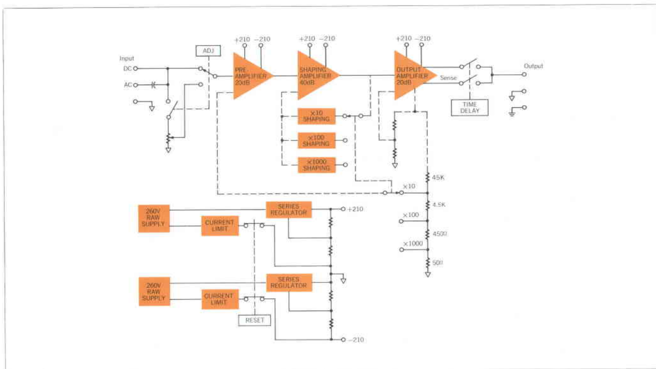
Fig. 2. Fixed gains in the -hp- Model 463A are selected by changing amplifier feedback characteristics by means of a precision feedback attenuator. The attenuator is made up of wire-wound resistors designed for good high-frequency characteristics, low temperature coefficient and good long-term stability.
