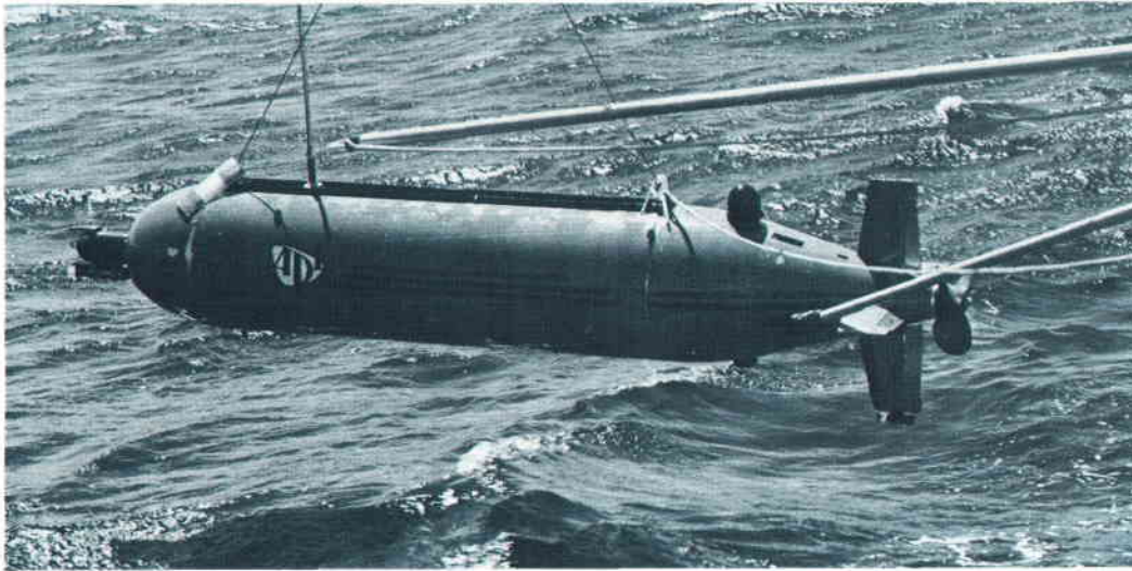
Fig. 6. Robot torpedo used by the Applied Physics Laboratory of the University of Washington for oceanographic research. A precision thermometer sensor mounted in the nose enables the vehicle to follow constant temperature lines through the water.
