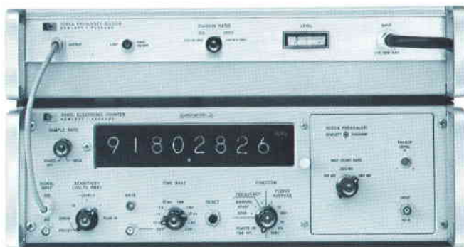
Fig. 1. Automatic Frequency Divider, -hp- Model 5260A, divides input frequencies between 0.3 GHz and 12.4 GHz by 100 or 1000 so they can be measured by a counter (counter shown is -hp- Model 5245L 50 MHz Counter). Divider operation is completely automatic except for selection of division ratio.
