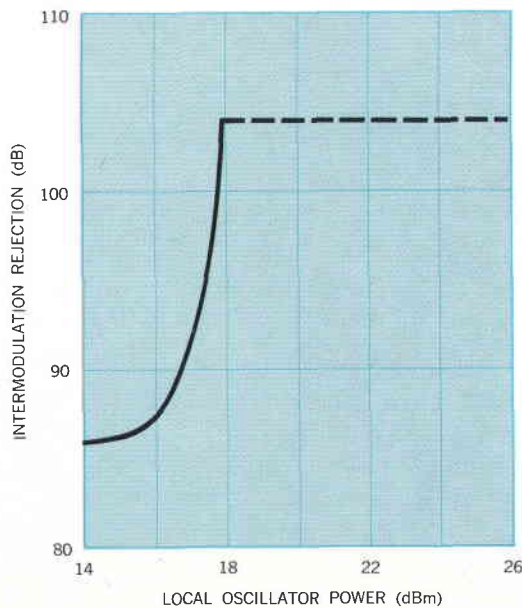
Fig. 3. IM rejection of a balanced hot-carrier diode mixer. Diode bias voltages were adjusted for best IM rejection at each LO level. For LO power above 18 dBm, maximum desired-signal power was used, and IM was below mixer noise level.
