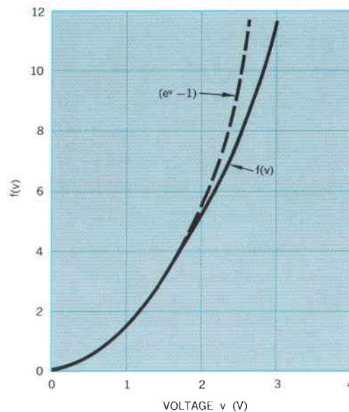
Fig. 4. Hypothetical diode characteristic used in text to illustrate cancellation of IM-producing higher-power coefficients of diode characteristics in balanced mixers.
