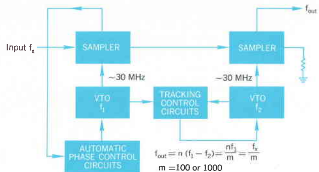
Fig. 2. Simplified block diagram of automatic frequency divider. Control circuits maintain indicated relationships between f_x , f_1 , and f_2 .
