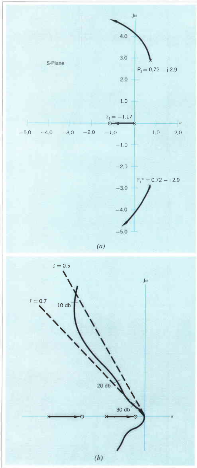
Fig. 4. (a). Magnified portion of root locus of main phase-lock loop. Note poles in right half plane which migrate to left half plane as loop gain increases. (b) Unmagnified root locus of main loop. Right-half-plane poles shown in (a) appear to start from origin on this plot. As loop gain increases by 30 dB, these poles move along line corresponding to damping ratios of 0.5 to 0.7. Thus loop is nearly critically damped over wide dynamic range.
