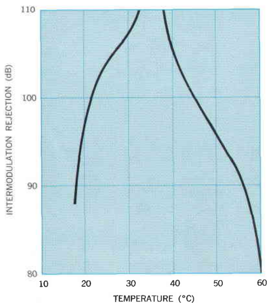
Fig. 6. Temperature dependence of IM rejection of a balanced hot-carrier-diode mixer.
