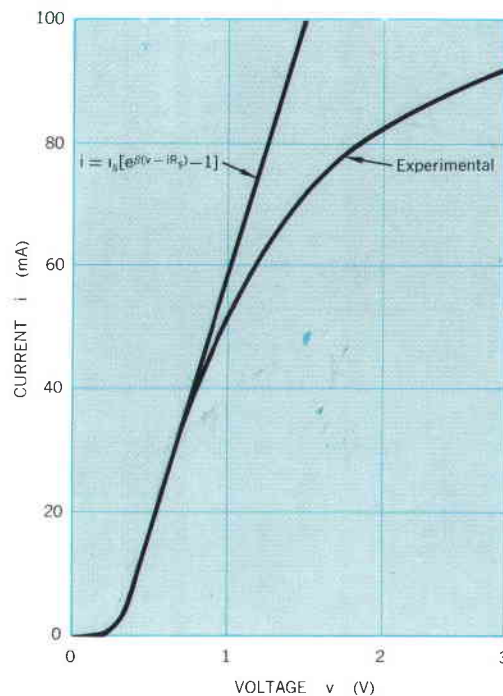
Fig. 1. Theoretical hot-carrier-diode curve and measured curve for typical hpa 2300-series diode.
