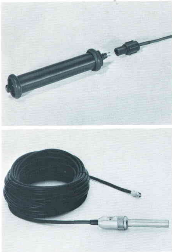
Fig. 3. A temperature sensing probe, the -hp- Model 2832A, top, houses the quartz crystal and all electronics in a pressure case designed specifically for measurement of ocean temperatures. At the bottom, the -hp- Model 2833A sensor assembly in a stainless steel case will withstand pressures to 10,000 psi and may be operated at distances up to one mile from the temperature readout.
