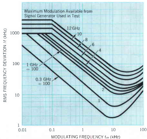
Fig. 5. Maximum frequency modulation on input signal that will permit frequency divider to lock on. These are typical measured characteristics at 0 dBm input. Division ratio was 1000 except where indicated.
