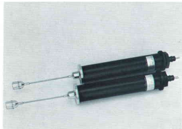
Fig. 5. Where a probe is used for precision measurements in still water, heat dissipated by the electronics in the package may heat the surrounding water, thus influencing the probe temperature. The modification shown here places the quartz crystal at some distance from the remainder of the probe and minimizes this effect.
