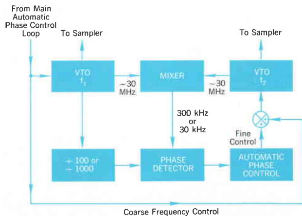
Fig. 3. Block diagram of tracking control used to keep frequency offset ( f_1 - f_2 ) equal to f_1/100 or f_1/1000 .
