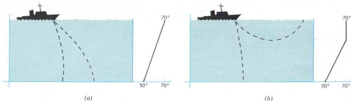
Fig. 1. Bending of a transmitted sonar beam (a) is caused by a combination of a gradual temperature change and a change in density of the water. At certain times of day, and after a storm, mixing occurs at the surface which results in a constant temperature zone. Under this condition, a sonar beam launched at an angle may return to the
