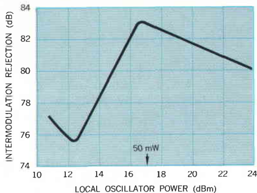
Fig. 2. Intermodulation rejection of a single-ended hot-carrier diode mixer. Diode bias was adjusted for best IM rejection at each local-oscillator level. IM rejection can be maximized by proper selection of diode bias and LO power, as explained in text.
