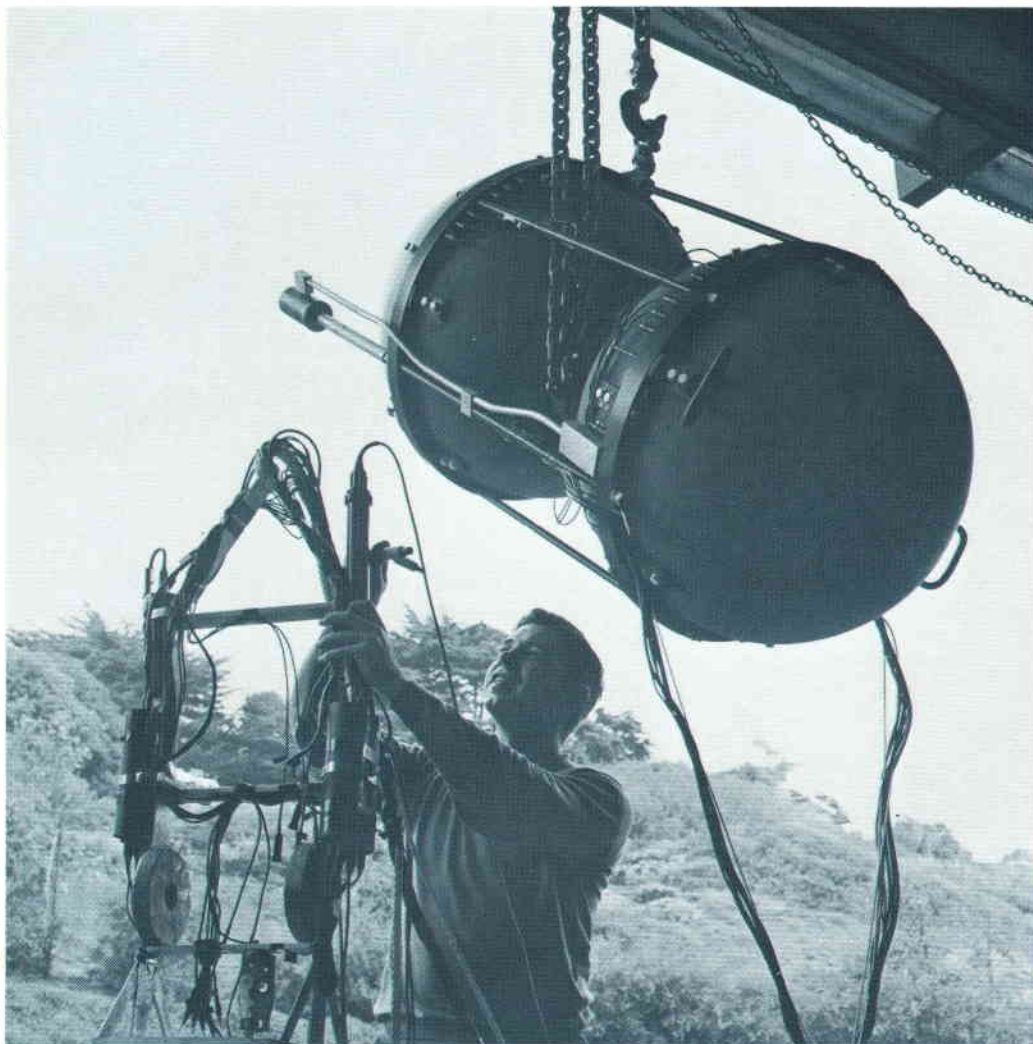
Fig. 2. Temperature sensor assembly is being mounted on an instrument tripod. It can be submerged to depths over 20,000 feet and can make temperature measurements to a resolution of 1/10 millidegree.
