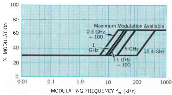
Fig. 6. Maximum amplitude modulation on input signal that will permit frequency divider to lock on. These are typical measured characteristics at 0 dBm input.
